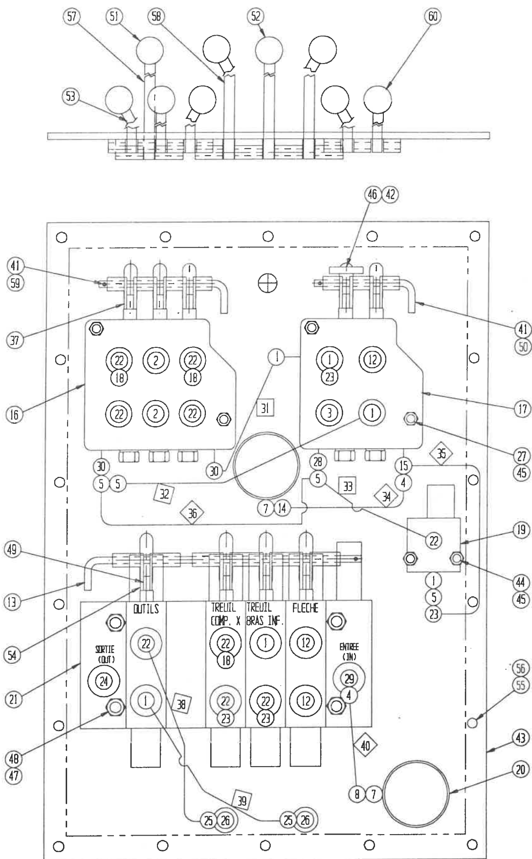
BASE DE CONTROLE AU SOL (FLOOR CONTROL AERA) (196-9661-004-00-2)
