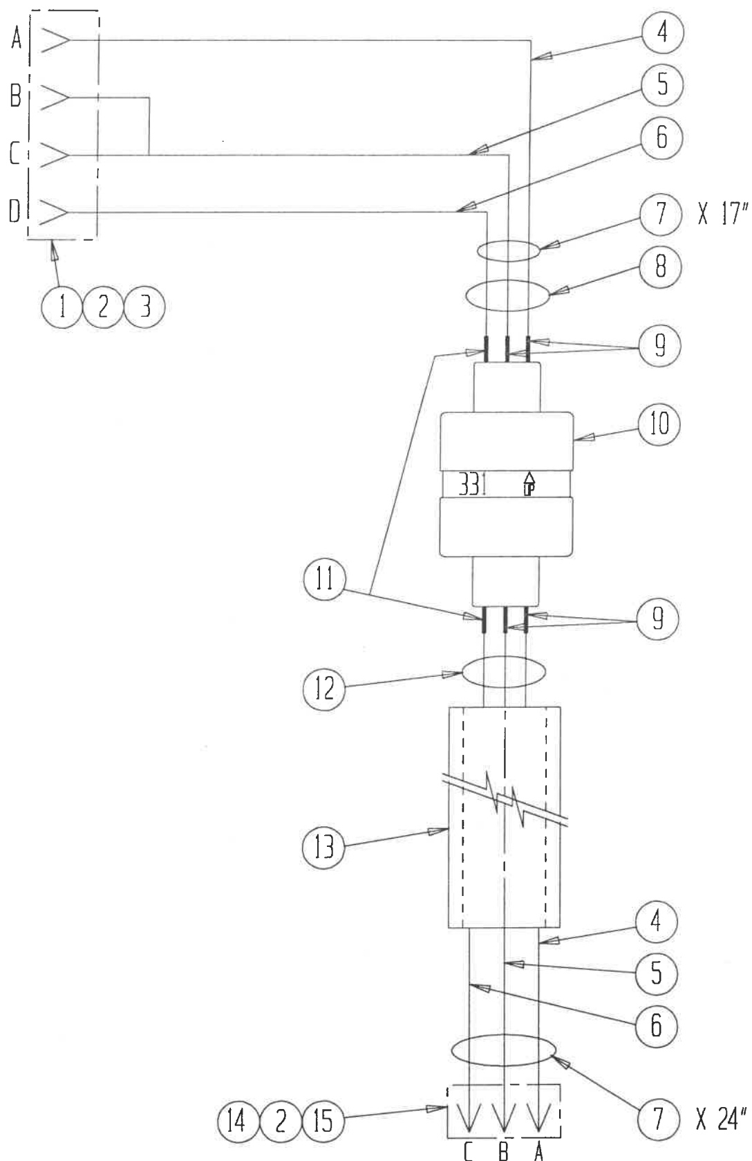
ROTATION CONTINUE ÉLECTRIQUE ASS'ÉE (ELECTRICAL CONTINUOUS ROTATION ASS'Y) (194-6625-001-00-2)
